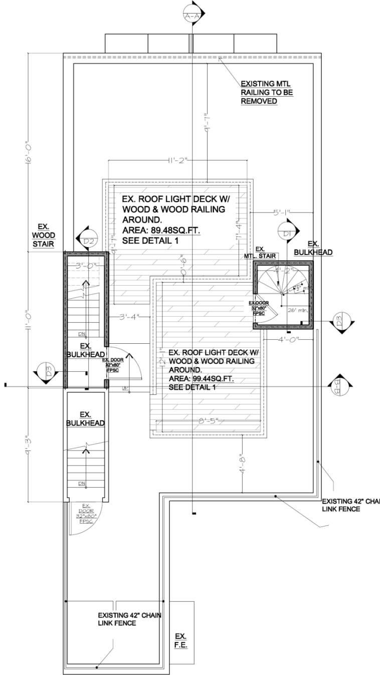
EXISTING ROOF FLOOR PLAN SCALE: 1/4" = 1'-0"
